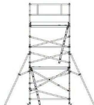
BASE UNIT & GUARD RAIL PACK WITH 2 x 1M EXTENSIONS Platform Height: 3.9m Reach Height: 5.9m
