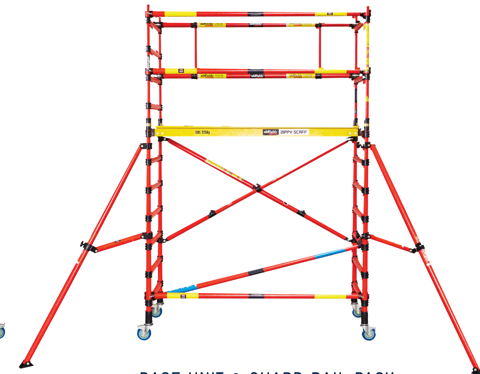
BASE UNIT & GUARD RAIL PACK Platform Height: 1.2m - 1.9m Reach Height: 3.6m - 3.9m BASE UNIT SKU: F-FSHA2 GUARD RAIL SKU: F-FSXP2
