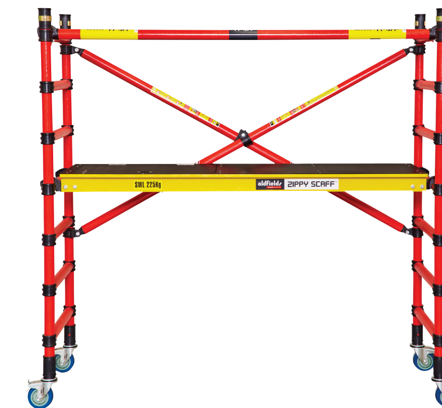
BASE UNIT Platform Height: 1.2m Reach Height: 3.2m BASE UNIT SKU: F-FSHA2
